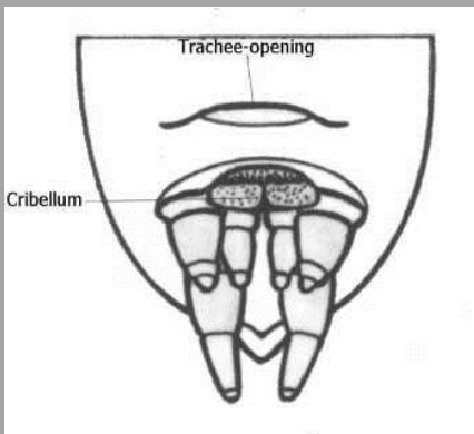
Cribellate spin
